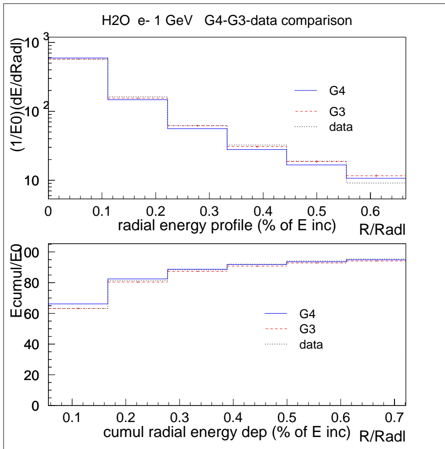
Fig. 6. Radial shower profile of E_0 = 1 GeV pencil electron beam in a cylinder of water, length 10 radiation lengths, radius 0.7 radiation lengths. The radial profile is the relative energy deposited per radiation length of radius. The cumulative profile is the energy deposited within a cylinder of given radius (the binning is 0.1 radiation lengths). Comparisons of GEANT4, GEANT3 and measurements are from [56]. G3 and G4 results are nearly identical.
