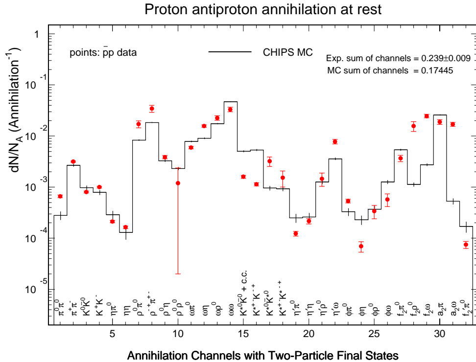
Fig. 11. Comparison of the branchings in two particle final states in proton anti-proton annihilation [100] with the predictions of CHIPS.
