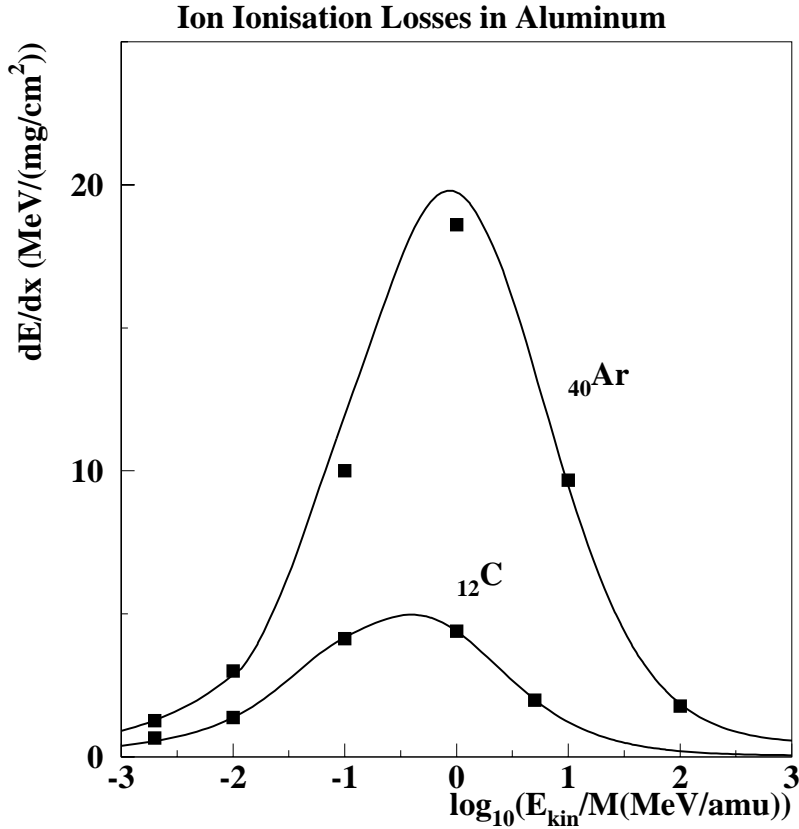
Fig. 8. Stopping power of Carbon and Argon ions in Aluminium as a function of the ion energy. Curves are GEANT4 simulation, points are evaluated data based on Ref. [72].
