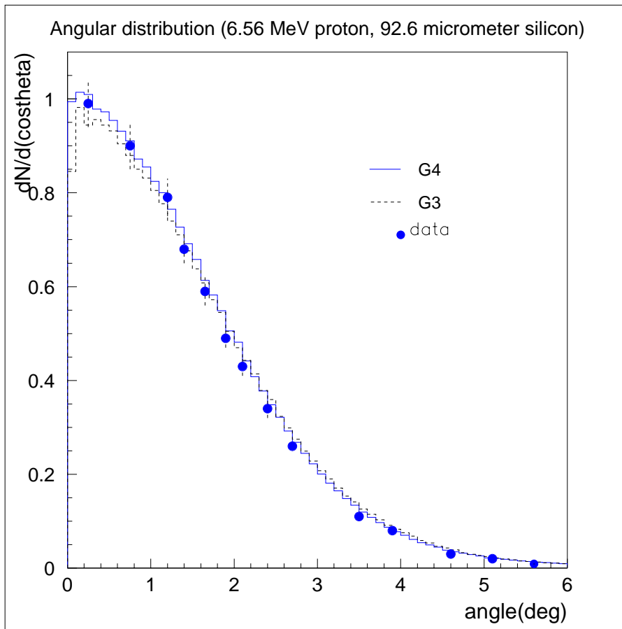
Fig. 5. Multiple scattering of 6.56 MeV protons by 92.6 \mu\text{m} of silicon: the angular distribution of exiting protons. Comparison of GEANT4, GEANT3 and data from [55]: G3 and G4 results are nearly identical, except at small angle.
