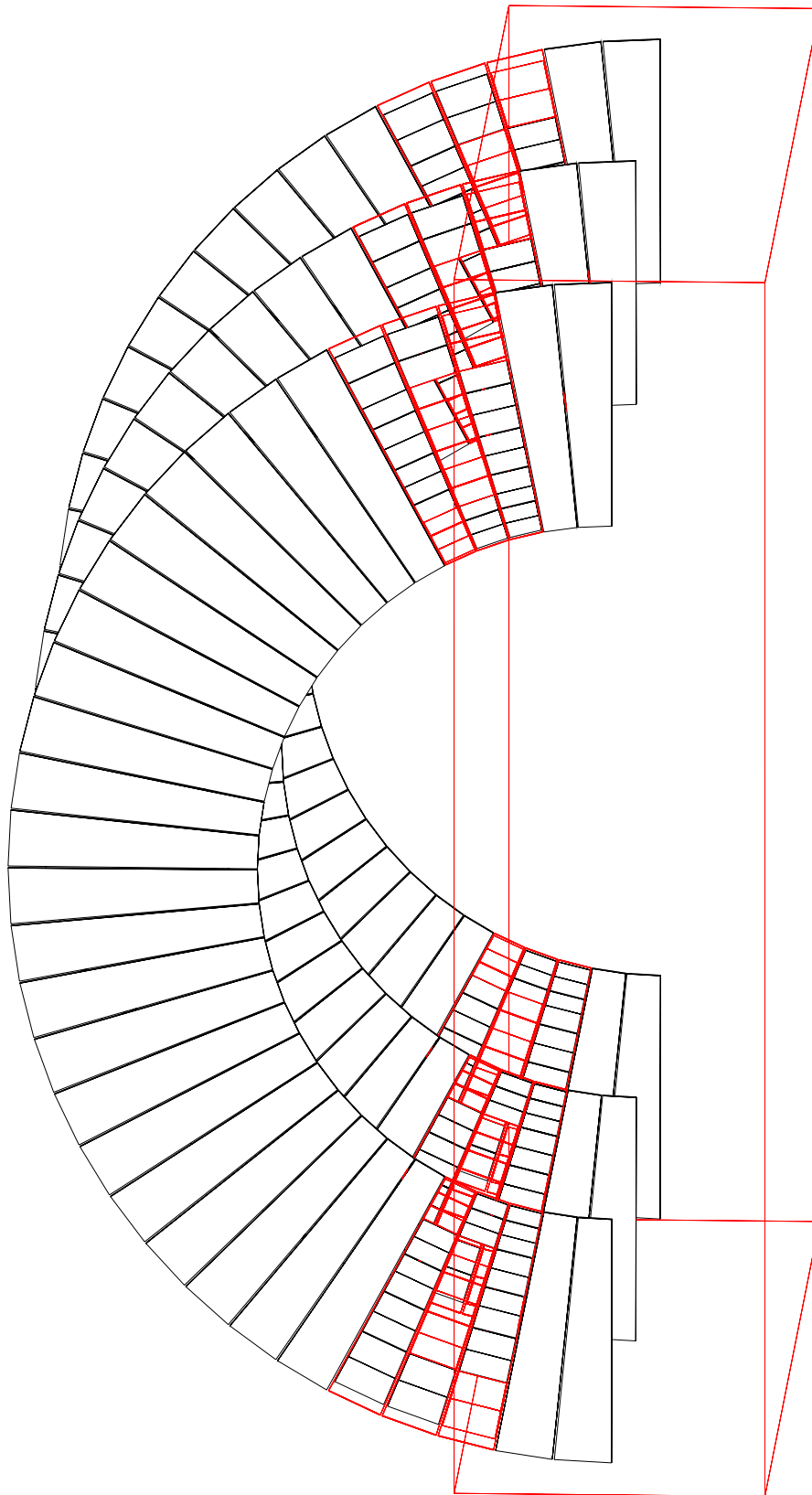
Fig. 15. Highlighting wrong intersections of physical volumes.
