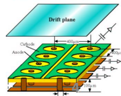
Micro Pixel Chamber
